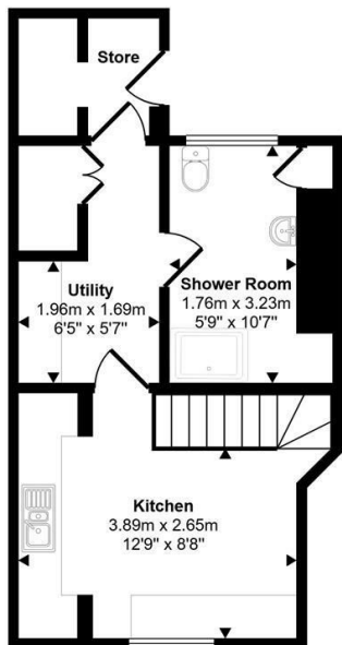
Lower Ground Floor Approx 33 sq m / 350 sq ft
